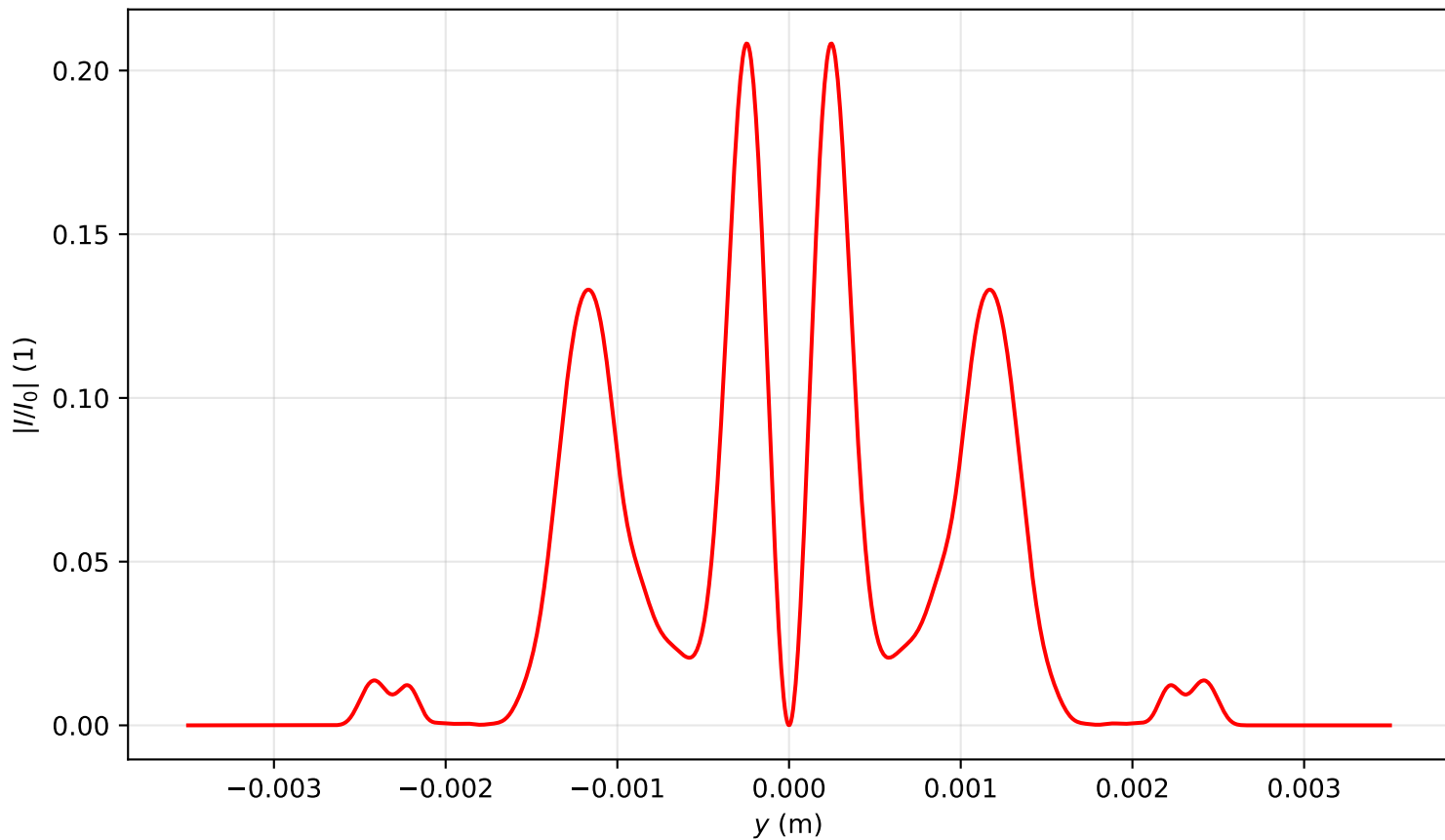
Intensity profile I(x=0, y, z=1.911)/I_0 , P_{in}=9.0P_{cr} , artificial time
